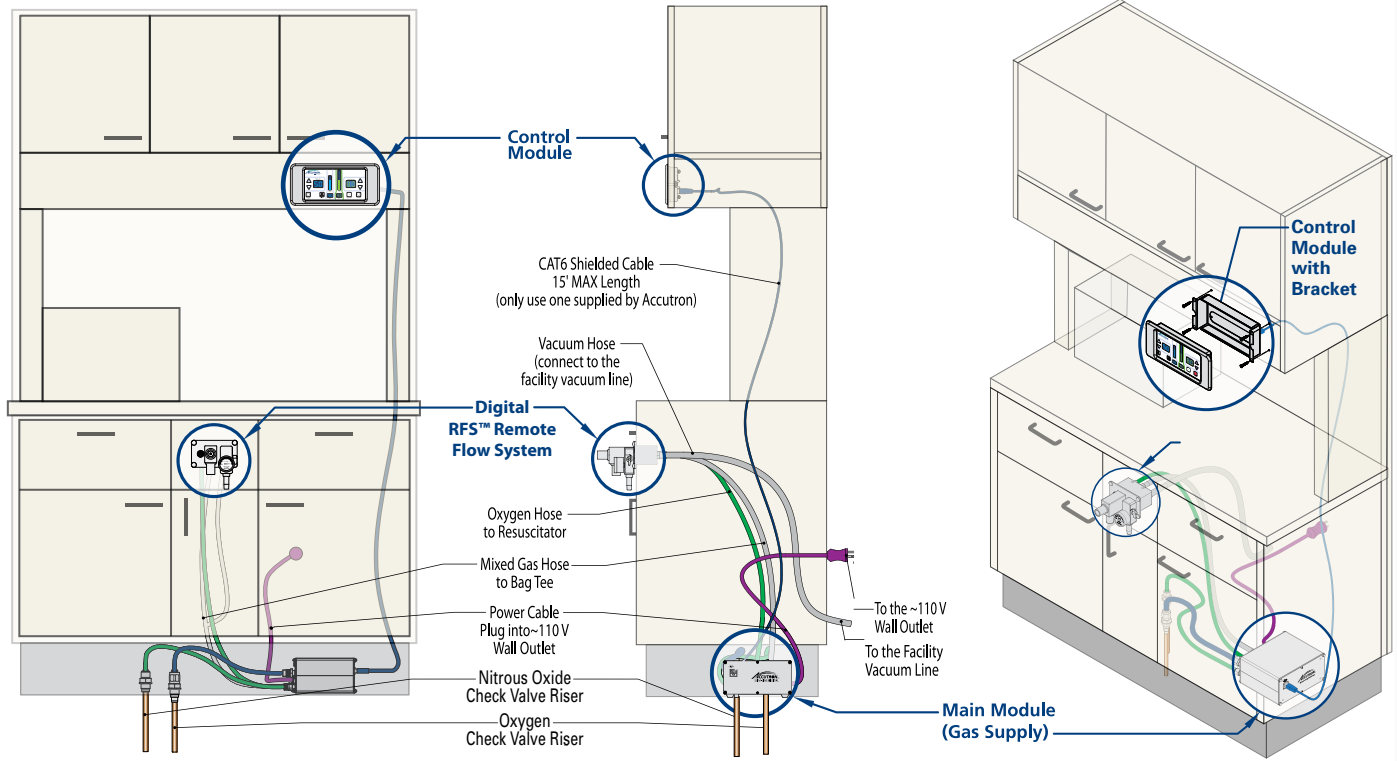
In-cabinet illustrations are specific to 56800 Digital Ultra® Flushmount with RFS™ Remote Flow System Vacuum Controller.
