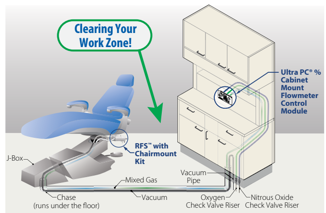
Ultra PC® % Cabinet Mount Flowmeter 36800-CHAIR 36800-CHAIR-NS
