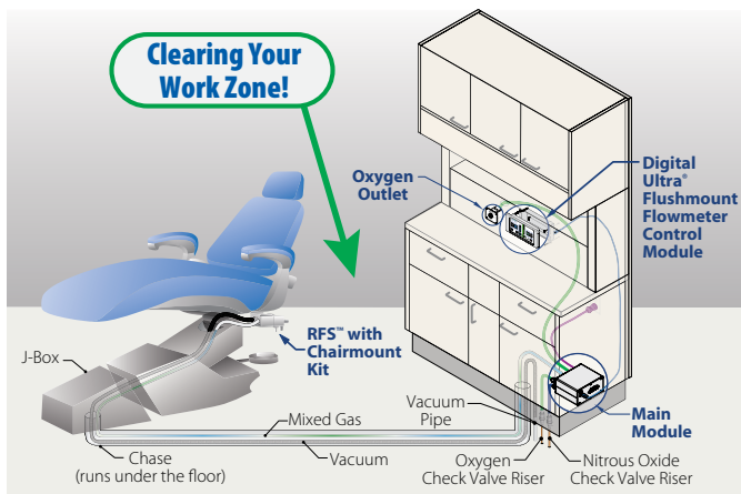
Digital Ultra® Flushmount Flowmeter 56800-CHAIR 56800-CHAIR-NS
